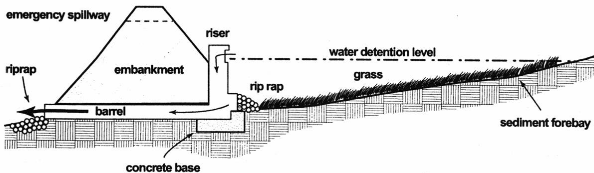
Figure 1: Typical Detention Pond Section
